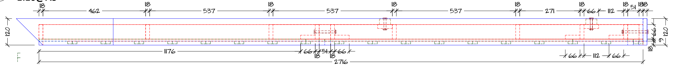
E.1.3 FRONT VIEW 1:10@A3
