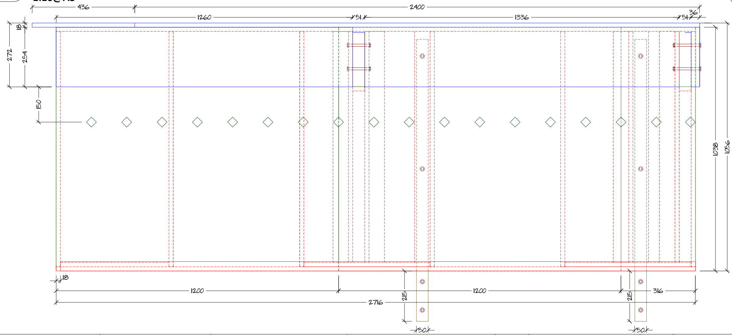
E.1.3 FRONT VIEW 1:10@A3
