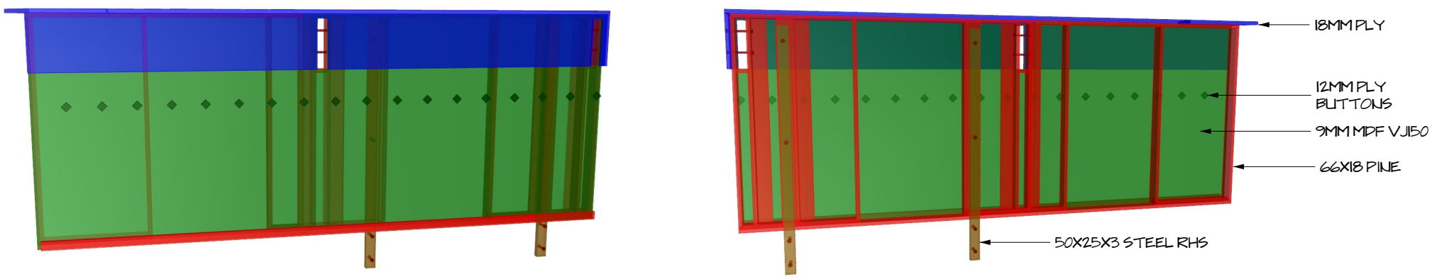
E.1.3 3D VIEWS NA@A3
