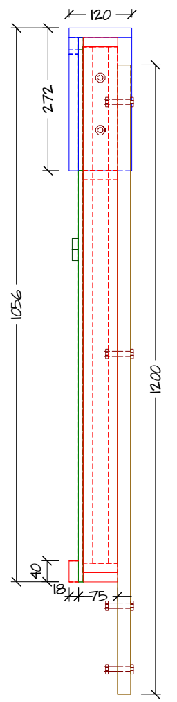
E.1.3 END VIEW 1:10@A3
